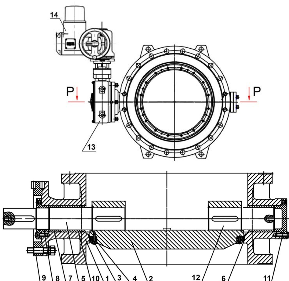
Section P-P
