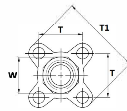
DN 1/4" - 3"
